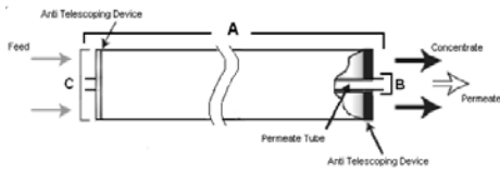
Figure 1a: Element Dimensions Diagram – Male
